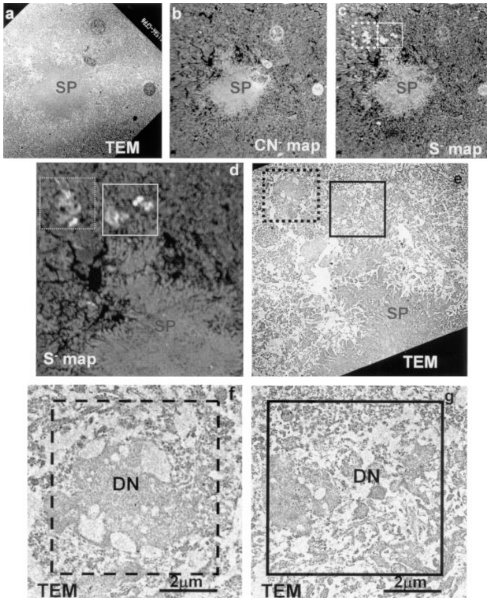
Fig. 4. Identification of S-rich structures in the periphery of senile plaques as dystrophic neurites. (a, e, f, and g) TEM images, (b–d) \text{CN}^- and \text{S}^- nanoSIMS maps at different magnifications. (a–c) [area of 50 \mu\text{m} \times 50 \mu\text{m} ]; (d–e) [area of 25 \mu\text{m} \times 25 \mu\text{m} ]. (f and g) detail of inset regions of (e) [area of 8 \mu\text{m} \times 8 \mu\text{m} ].
